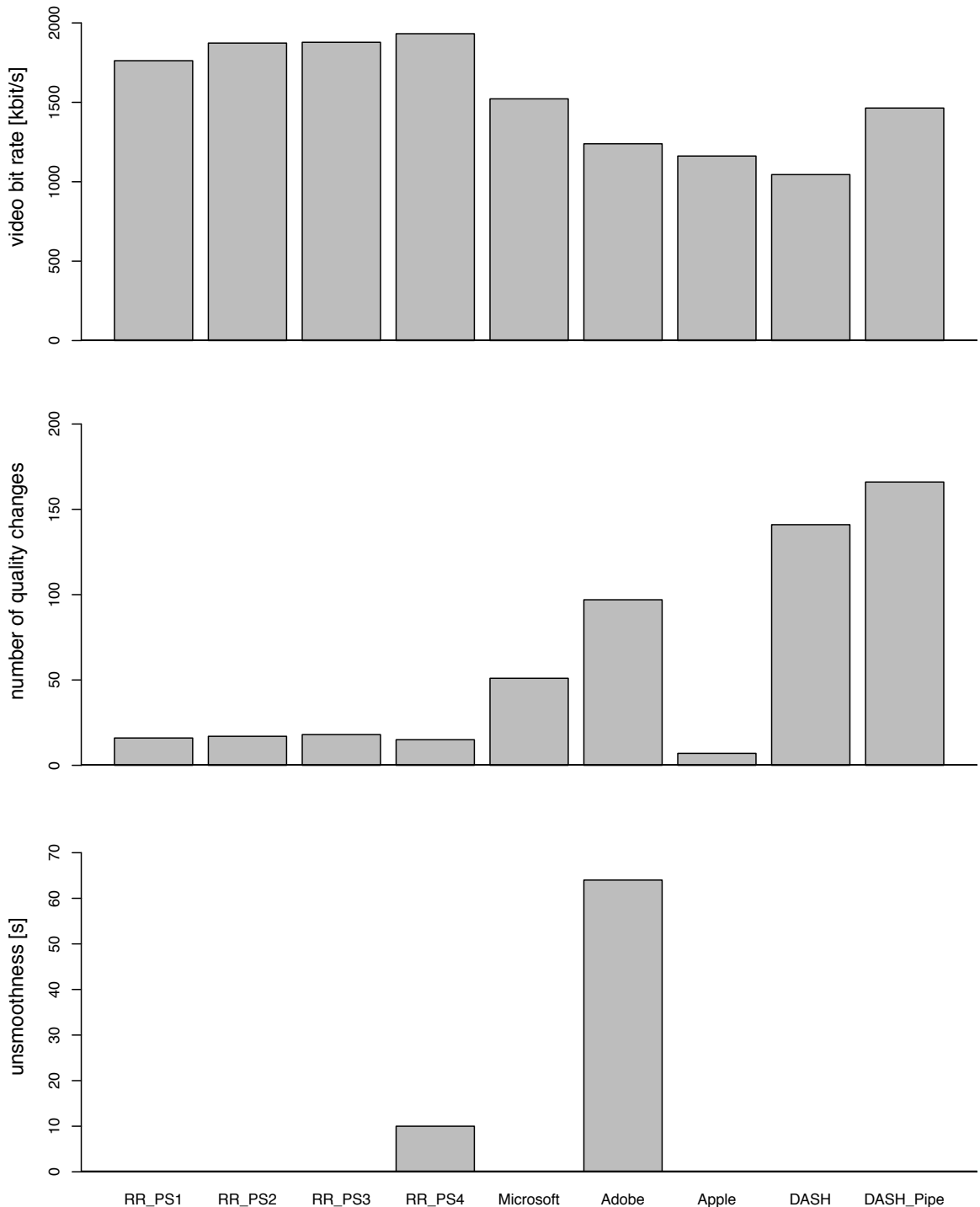
Figure 8.16: Average video bit rate, number of quality switches and unsmoothness of the request-response (RR) streaming system ( t_{frag} = 30 seconds) and adaptive streaming systems evaluated in [66], averaged over all network traces.
