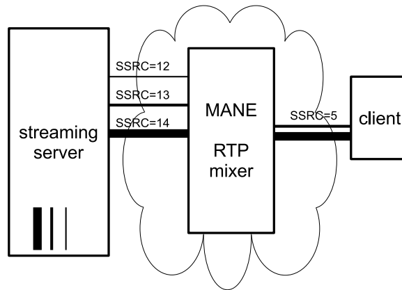
Figure 4.7: Simple RTP mixer [54].
