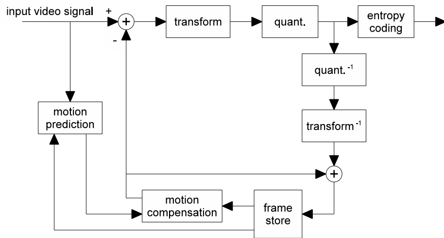
Figure 2.1: Example of a hybrid video coding approach of inter-frame prediction and transform coding.
