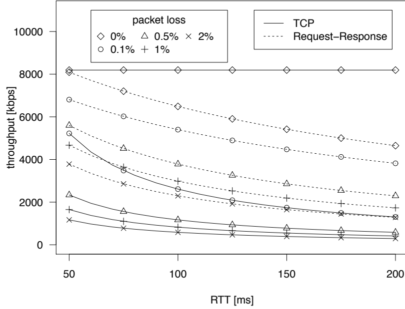
Figure 6.6: Modeled throughput performance of a single TCP connection (TCP) r_{tcp} and the request-response streams r_{rr} ( MSS = 1460 bytes, l_{ch} = 160 kB, n_c = 5 , t_{gap} = 210 ms) at a fixed bottleneck bandwidth BW = 8192 kbps and packet loss rate p [53].
